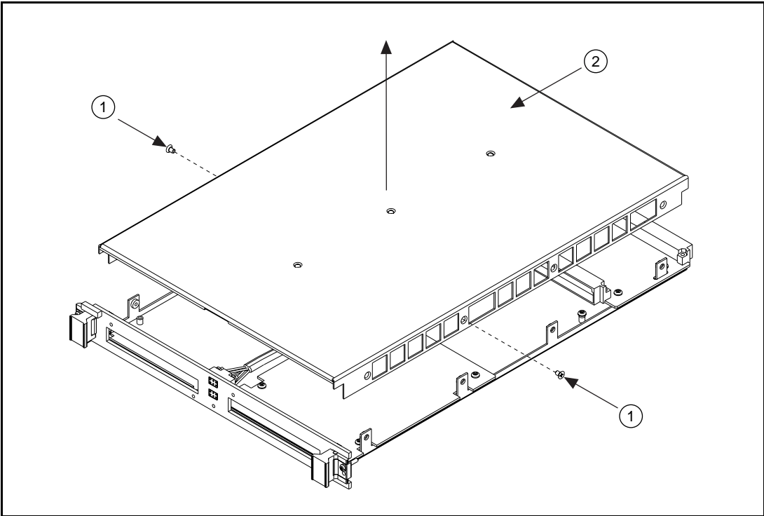
1 No. 4-40 x 3/16 in. Flathead Screws 2 Top Cover
