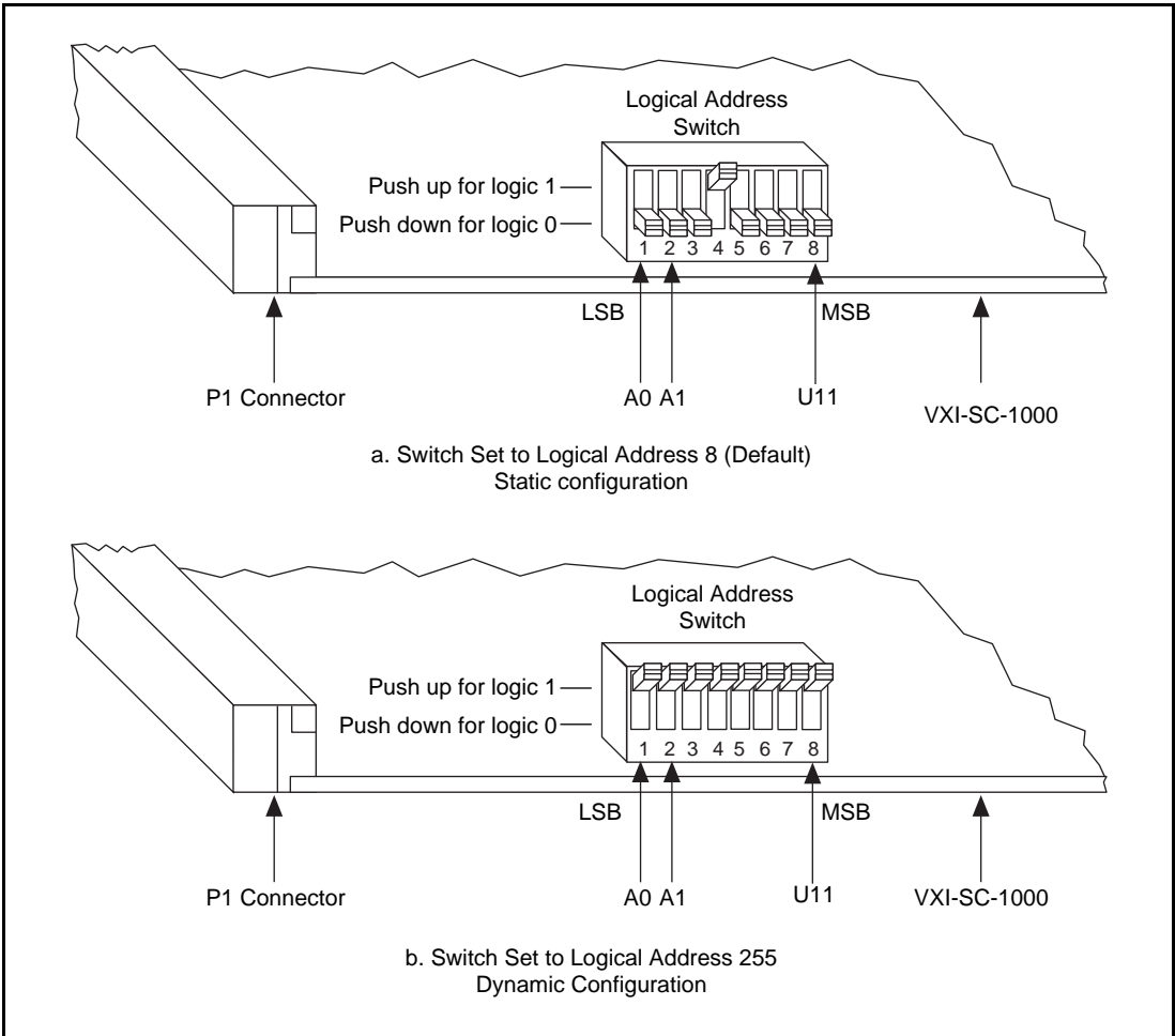
Figure 9. VXI-SC-1000 Logical Address Selection
