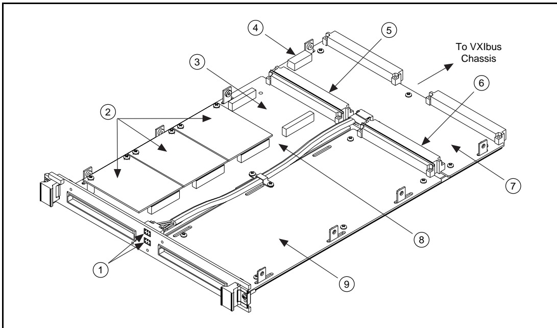
Figure 1. Components of a VXI Signal Conditioning System
